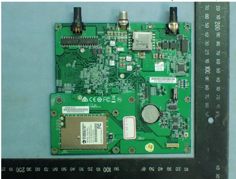
Figure 11 Internal View (Main Board, Front View)
