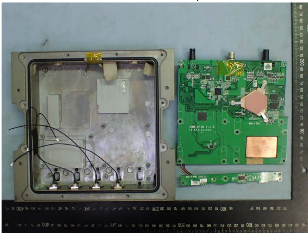
Figure 8 Internal View (Removed Internal Main Board)
