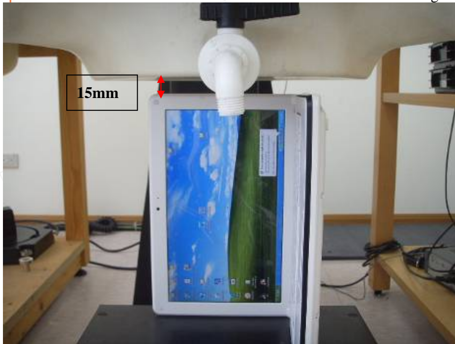
Fig.5 Right side of Notebook is paralleled with flat phantom, and spacing between EUT and Phantom is 15mm.
