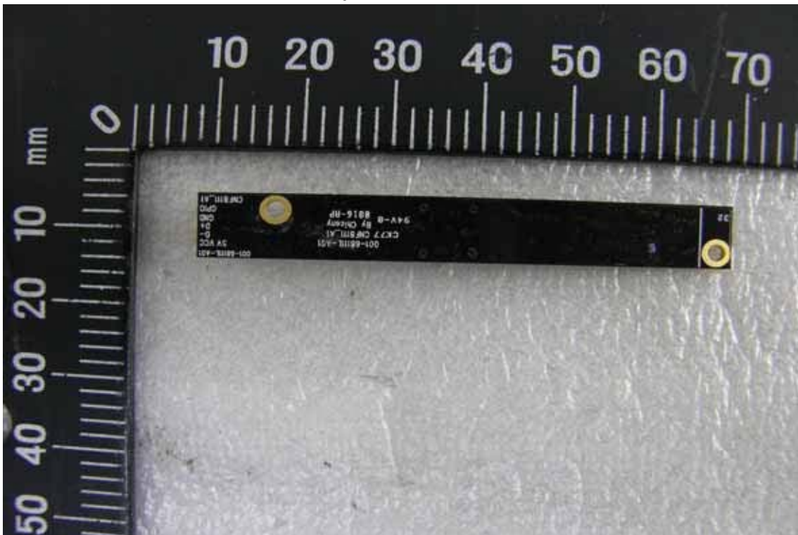
Internal of EUT – 17 (Webcam)
