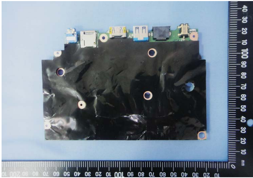
(20)EUT Photo
