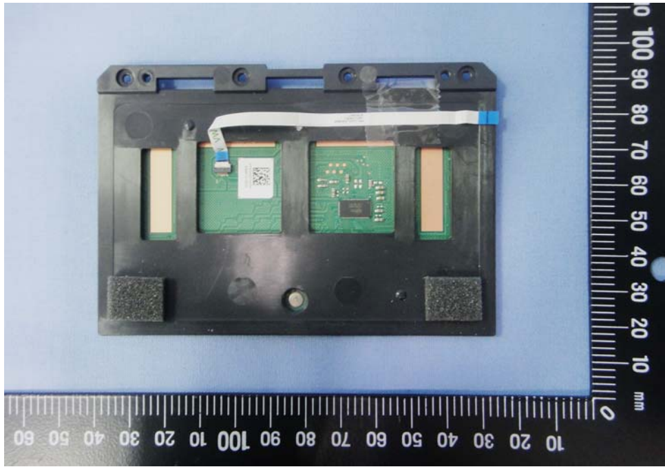
(26)EUT Photo
