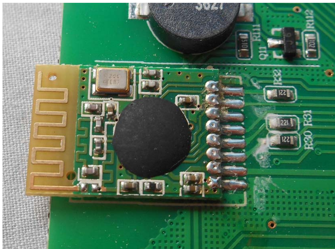
FIGURE 4 REMOTE CONTROLLER (M/N: SFD-Y-14) RF MODULE (FRONT SIDE)
