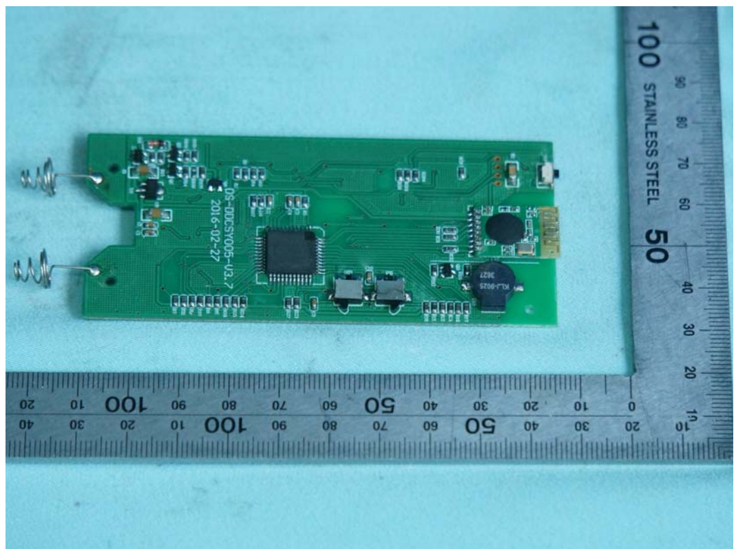
FIGURE 8 REMOTE CONTROLLER (M/N: SFD-Y-18) MAIN BOARD (COMPONENT SIDE)
