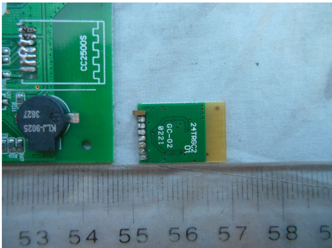
FIGURE 6 REMOTE CONTROLLER (M/N: SFD-Y-14) RF MODULE (BACK SIDE)
