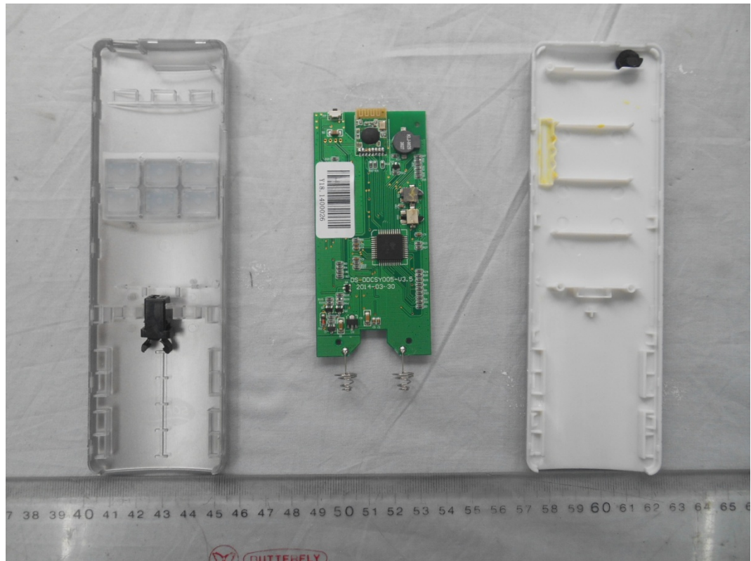
FIGURE 7 REMOTE CONTROLLER (M/N: SFD-Y-18) COVER REMOVED
