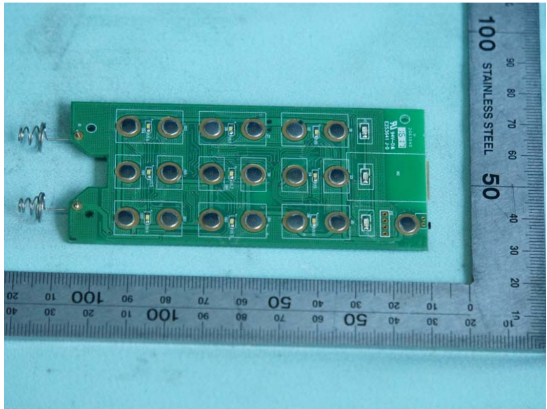
FIGURE 9 REMOTE CONTROLLER (M/N: SFD-Y-18) MAIN BOARD (SOLDERED SIDE)
