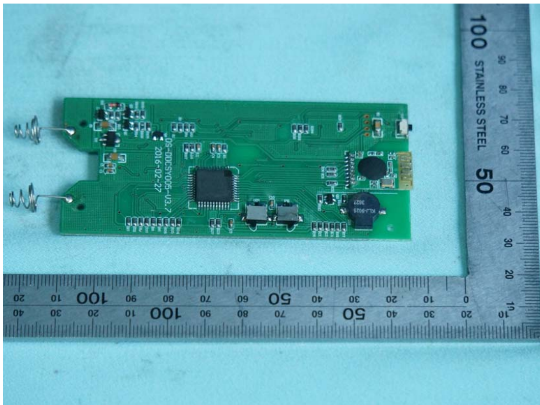
FIGURE 2 REMOTE CONTROLLER (M/N: SFD-Y-14) MAIN BOARD (COMPONENT SIDE)
