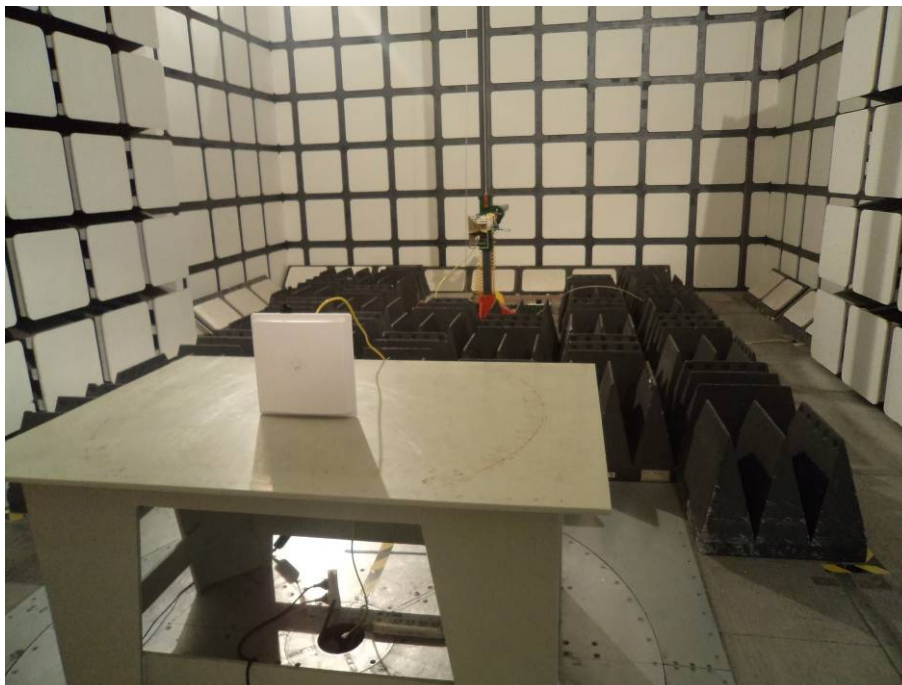
Radiated Emissions View (1-10 GHz)
