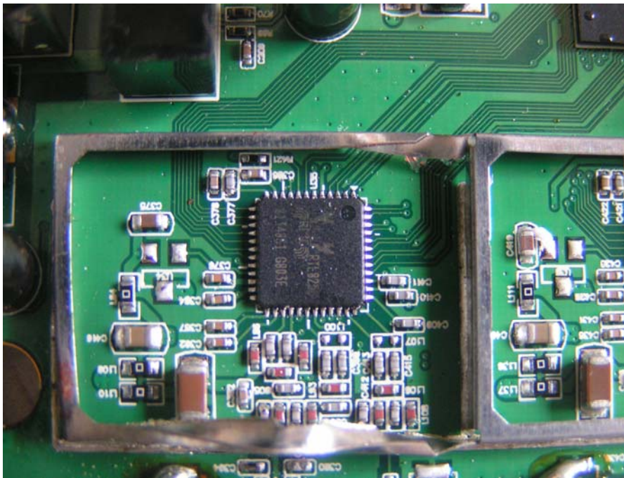
RF Module #2 View
