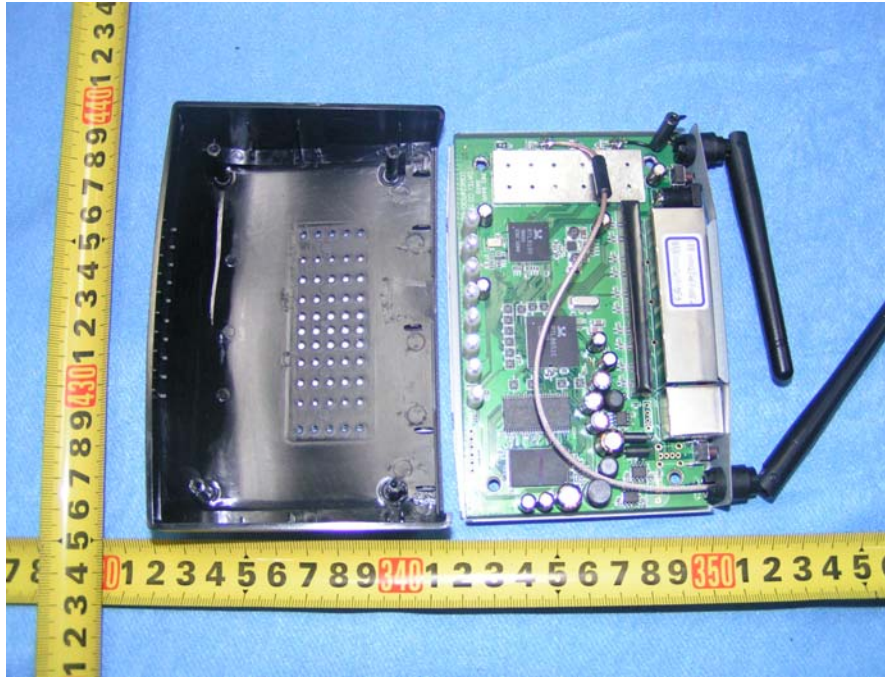
Cover Removed View
