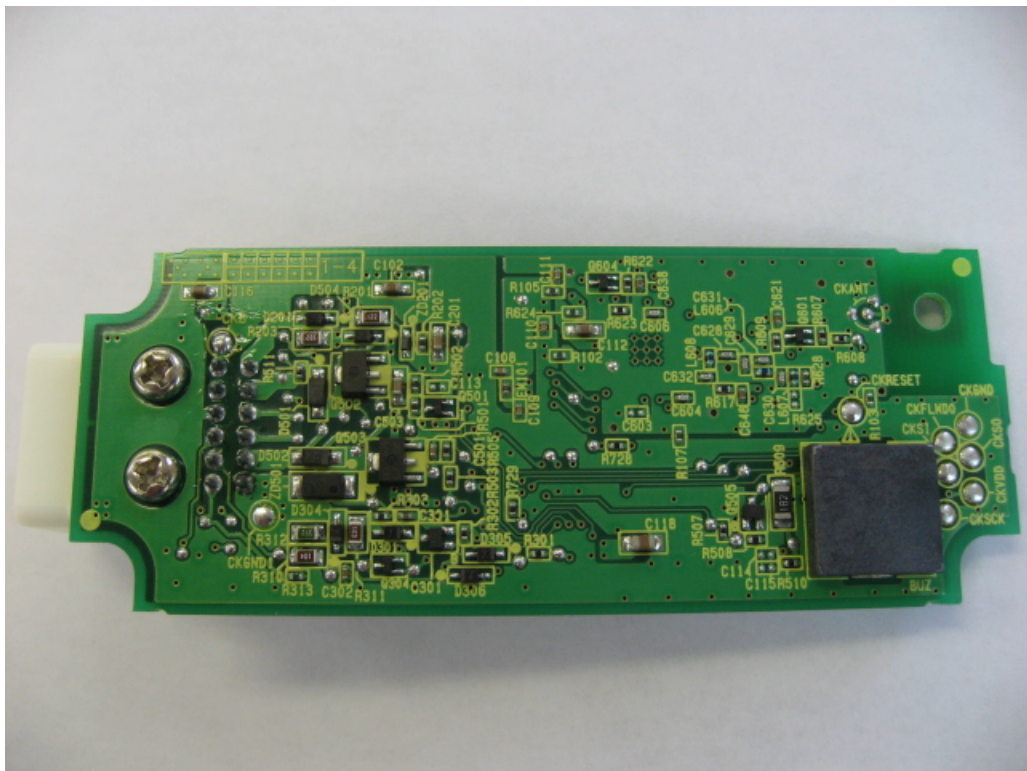
Bottom view of RES ECU circuit board
