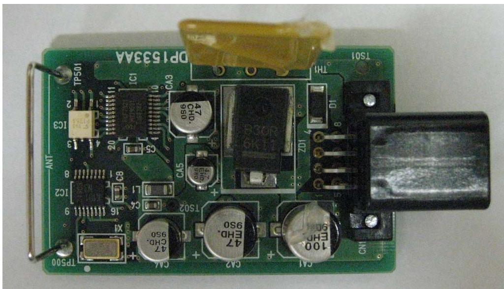
Fig .2 Top view of Remote Controller circuit board There are some parts below the thermistor.
