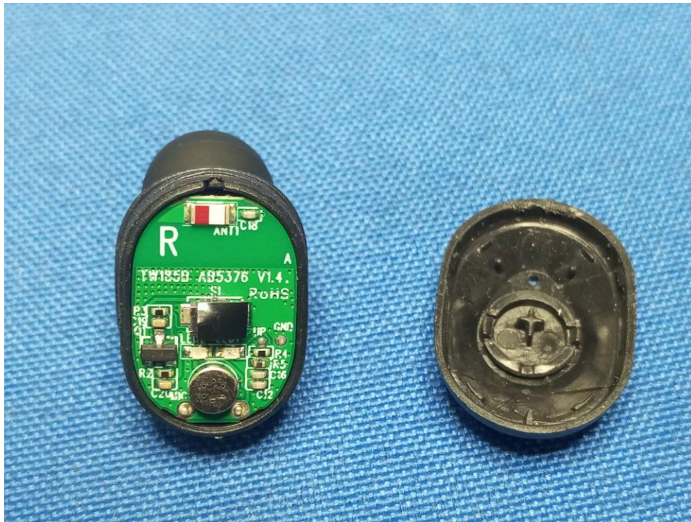
Right earphone
