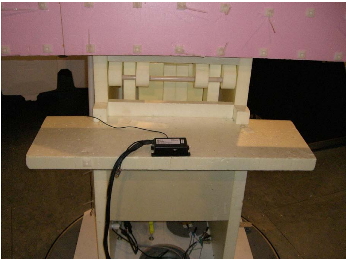
FCC Part 15B Radiated Emissions <1GHz
