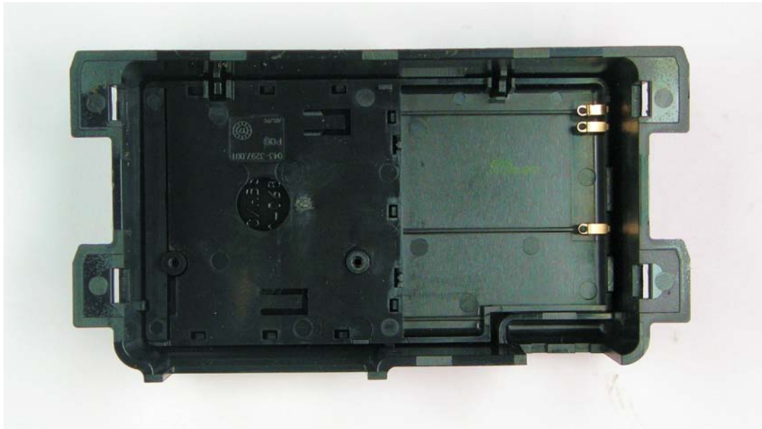
Inside housing (top) with internal GSM antenna
