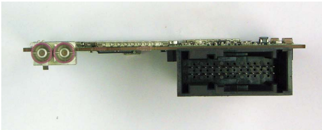
PWB side view with GPS antenna connector, external GSM antenna connector and system connector
