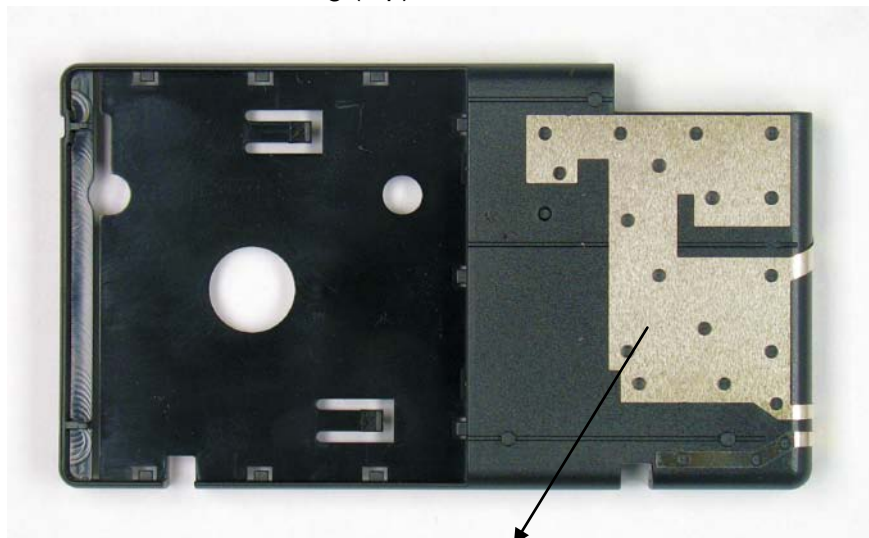
Internal GSM antenna (top view)
