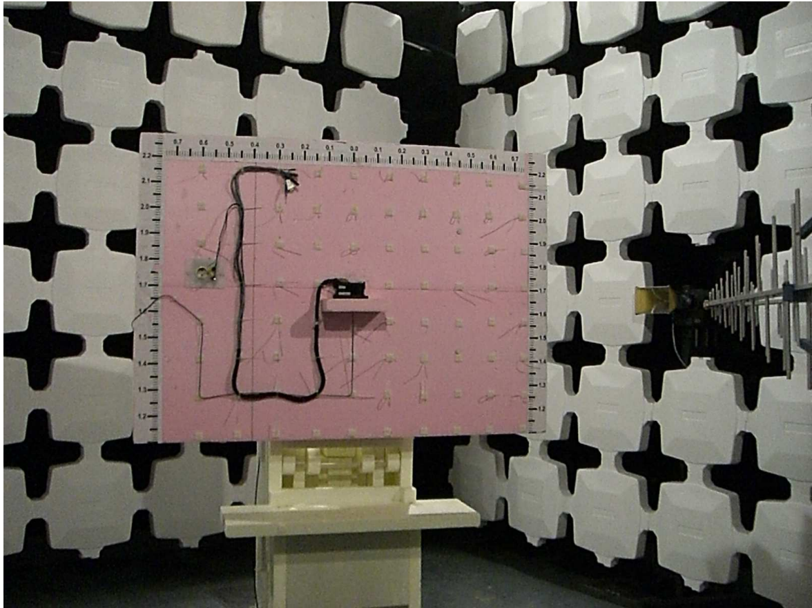
FCC Part 22/24/27 Radiated Emissions Test Setup
