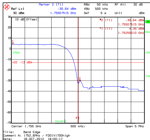
Channel 1432 / 1752.6 MHz
