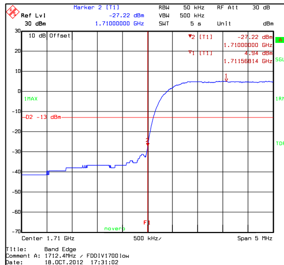
Channel 1392 / 1712.4 MHz
