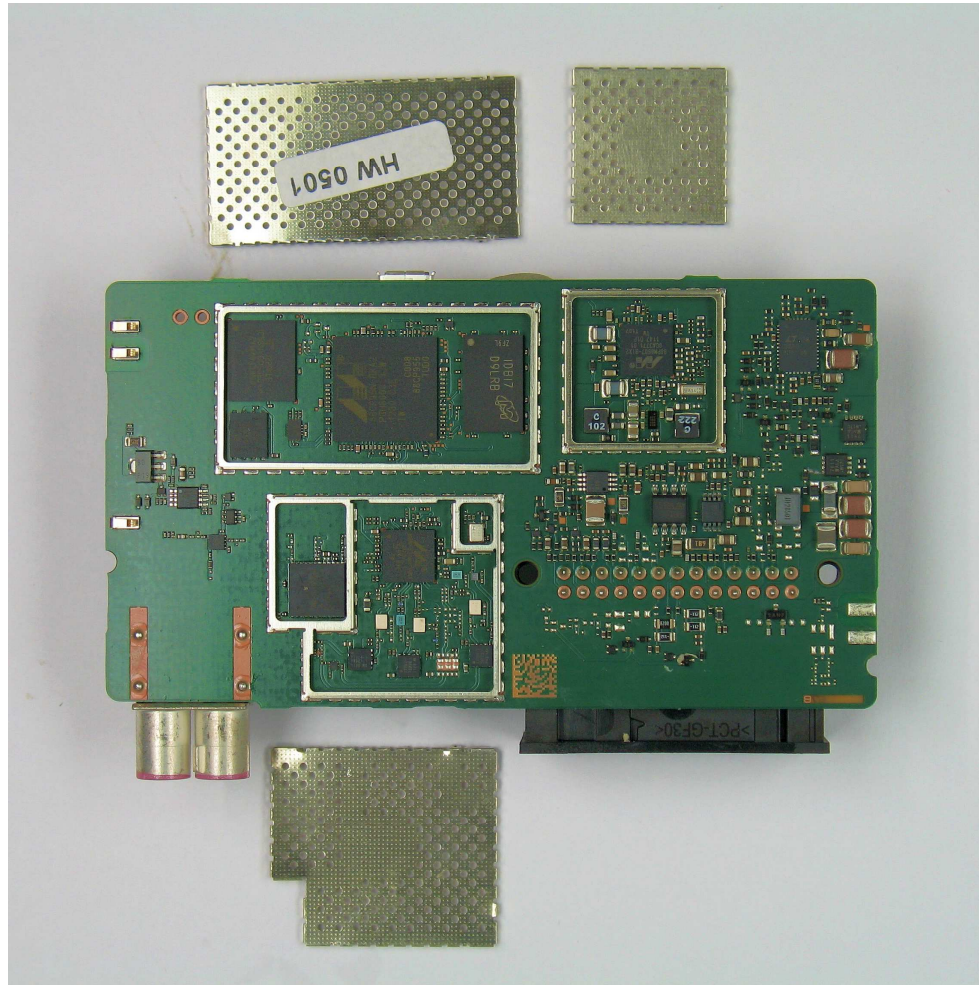
Bottom view of PWB without shields
