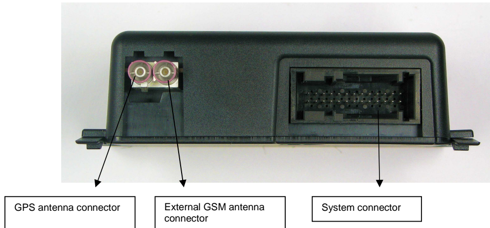
Side view with external GSM antenna connector, GPS antenna connector and system connector
