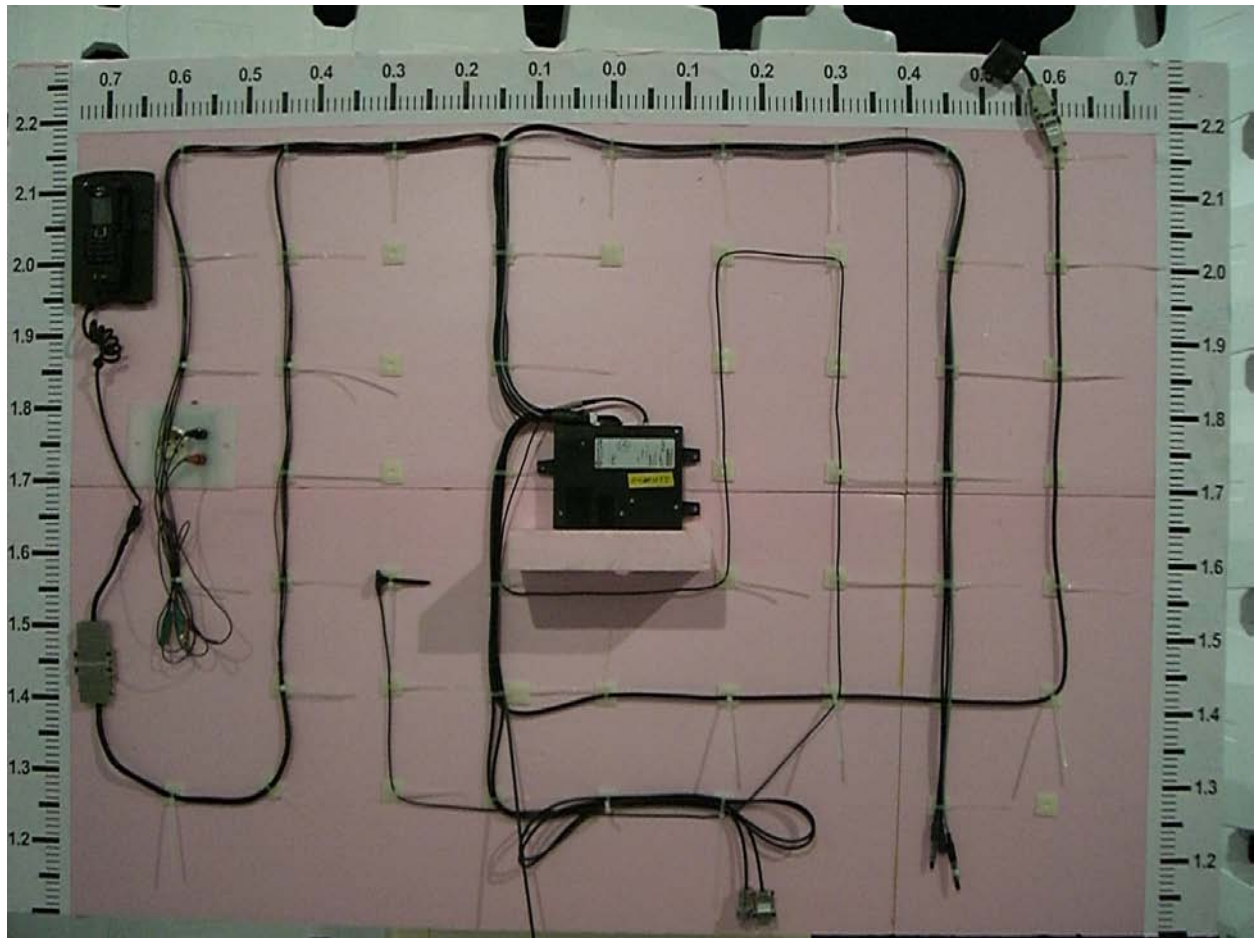
FCC Part 15C/22/24 Radiated Emissions Test Setup
