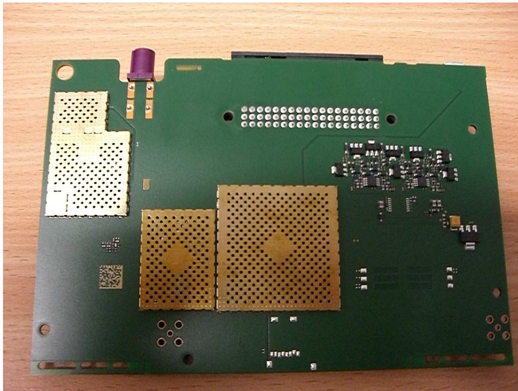
Bottom View of PWB with shields
