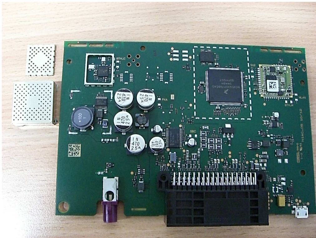
Top View of PWB without shields
