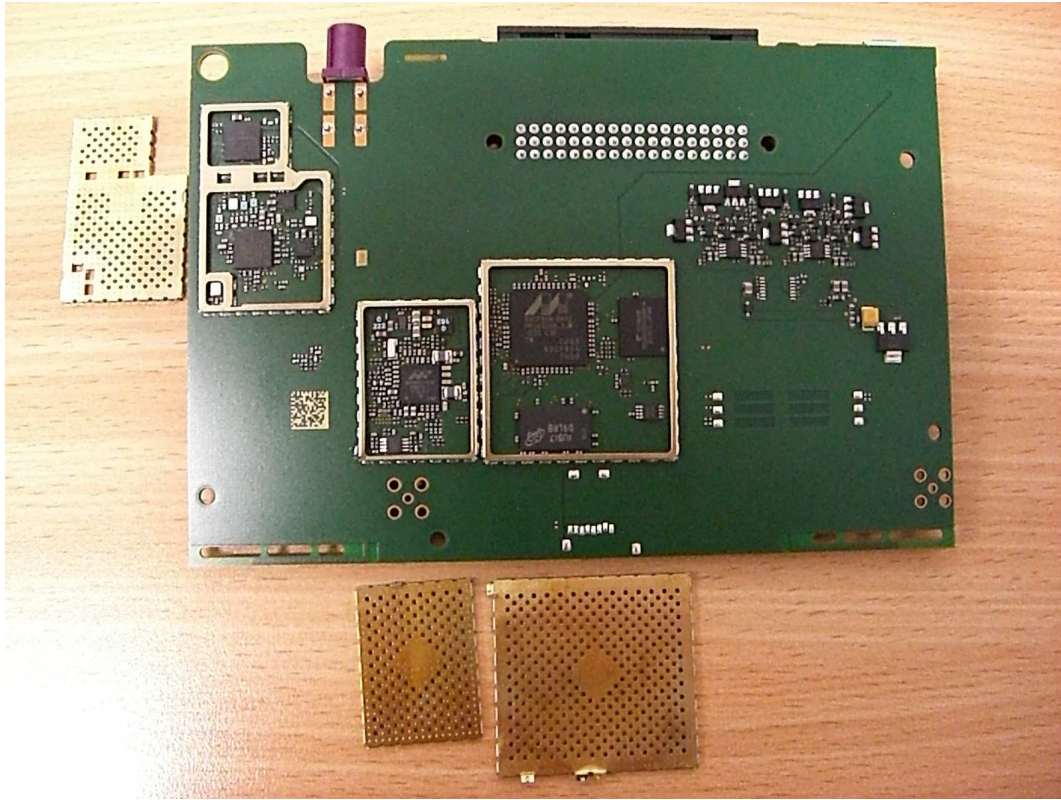
Bottom View of PWB without shields
