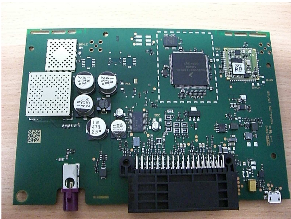
PWB inside housing
