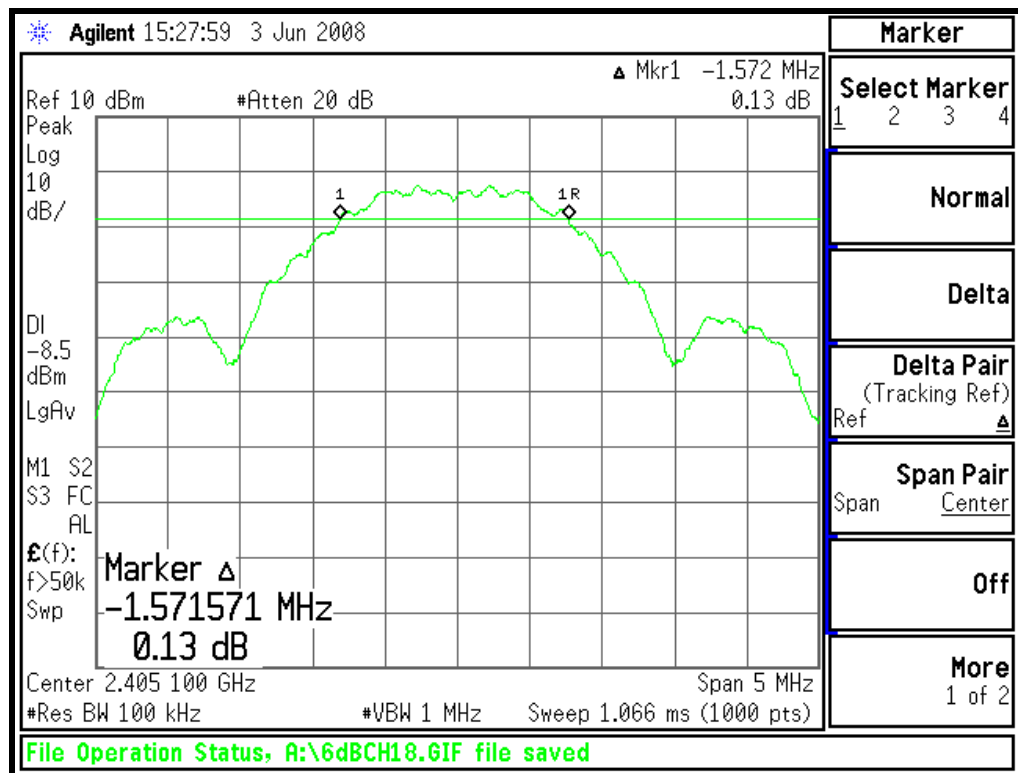
6dB Bandwidth: Channel 11
