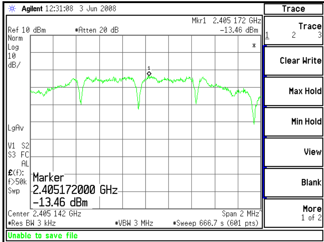
Power Spectral Density: Channel 11
