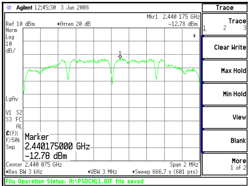
Power Spectral Density: Channel 18
