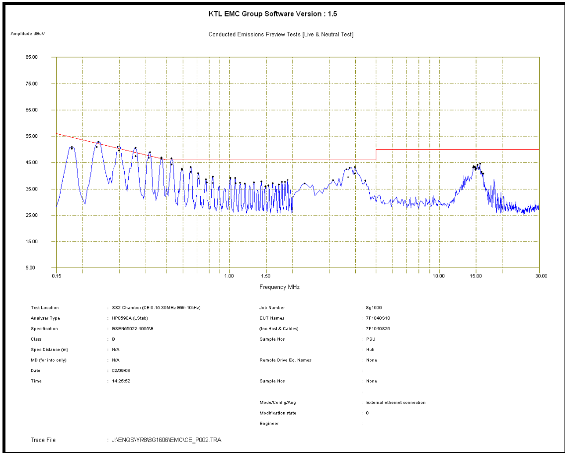
Power Line Conducted Emissions
