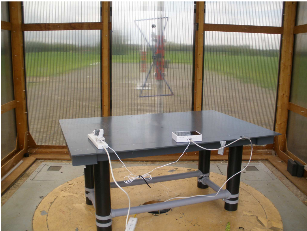
Photograph 4 Radiated Emissions - Flat - Back
