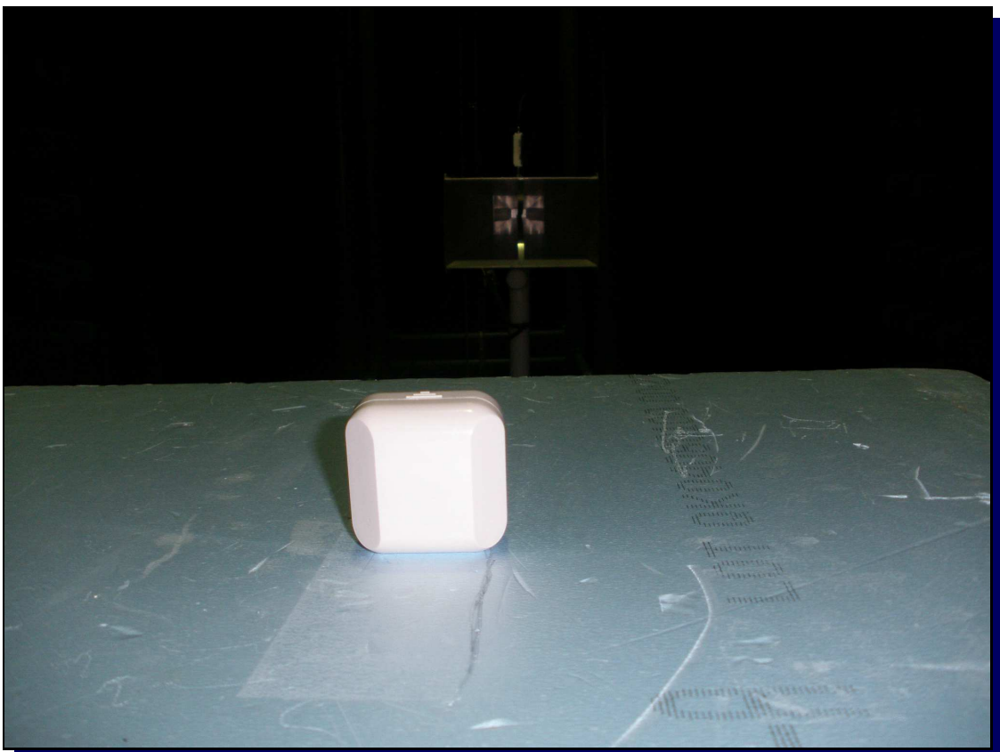
Photograph 2 Radiated Emissions - Upright - Back
