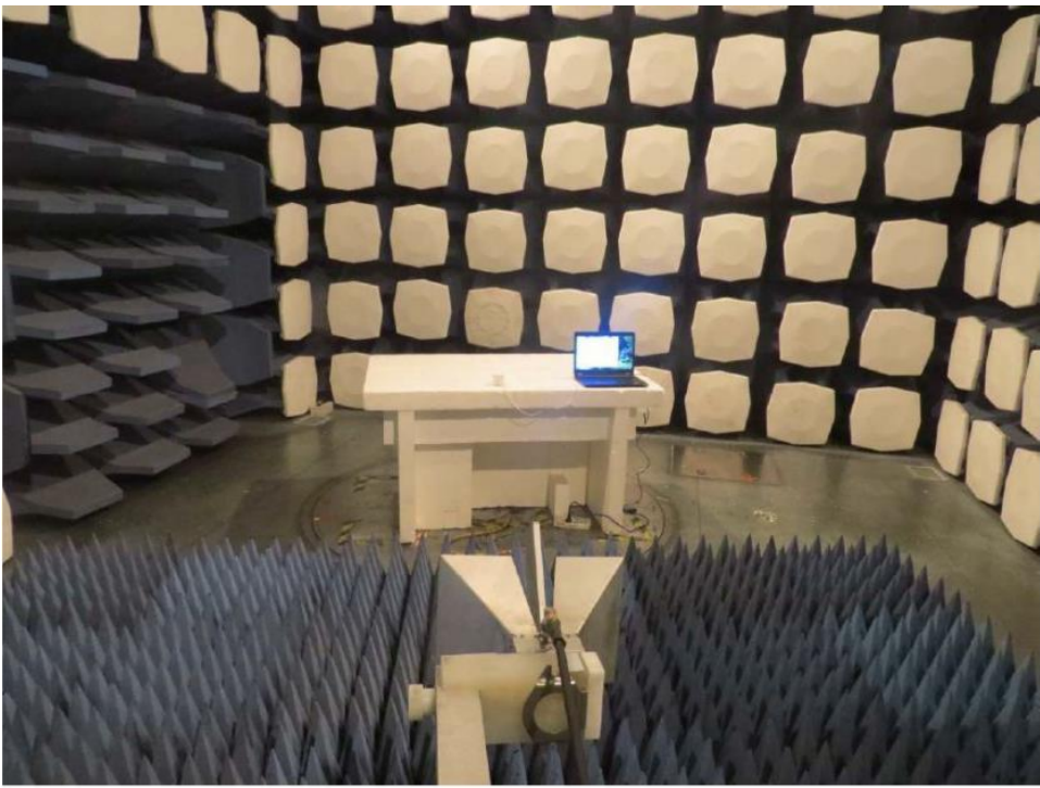
Radiated Emission (above 1GHz) of transfer data mode
