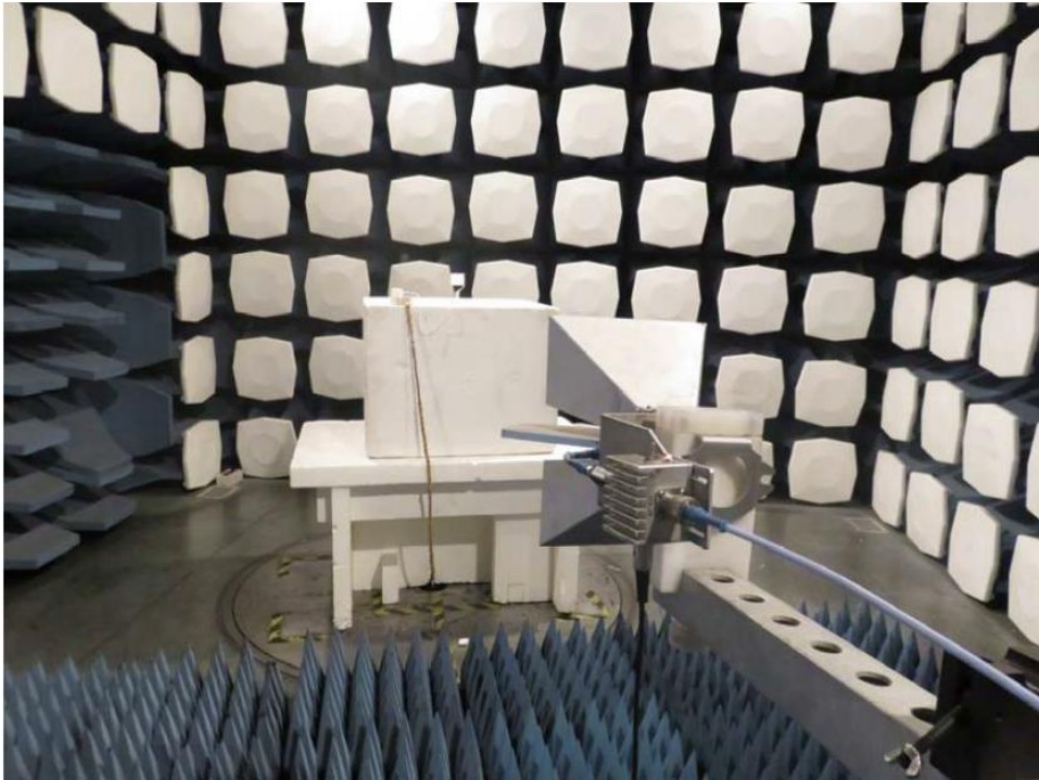
Radiated Emission (Above 1GHz) of wireless transmit mode
