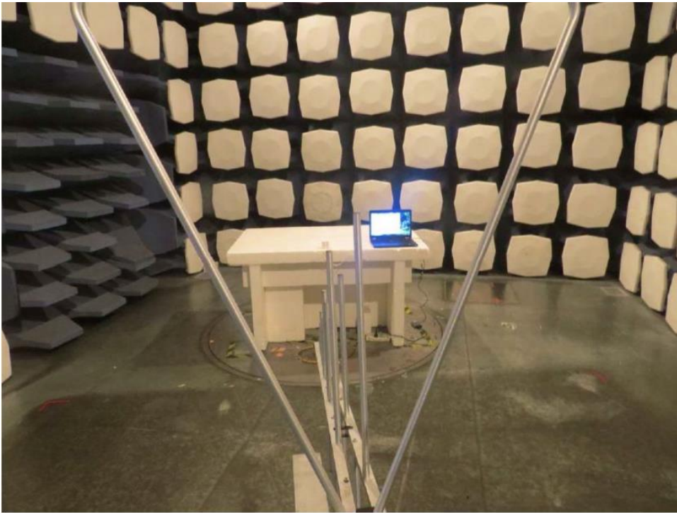
Radiated Emission (30MHz-1GHz) of transfer data mode
