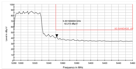
802.11ac HT20 -Channel 64: Peak
