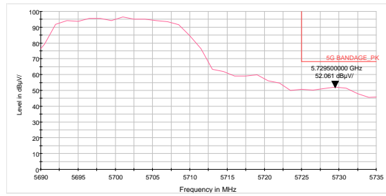
802.11a-Channel 140: Peak
