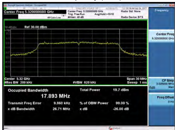
U-NII-2A, 802.11ac HT20 Carrier frequency (MHz): 5320
