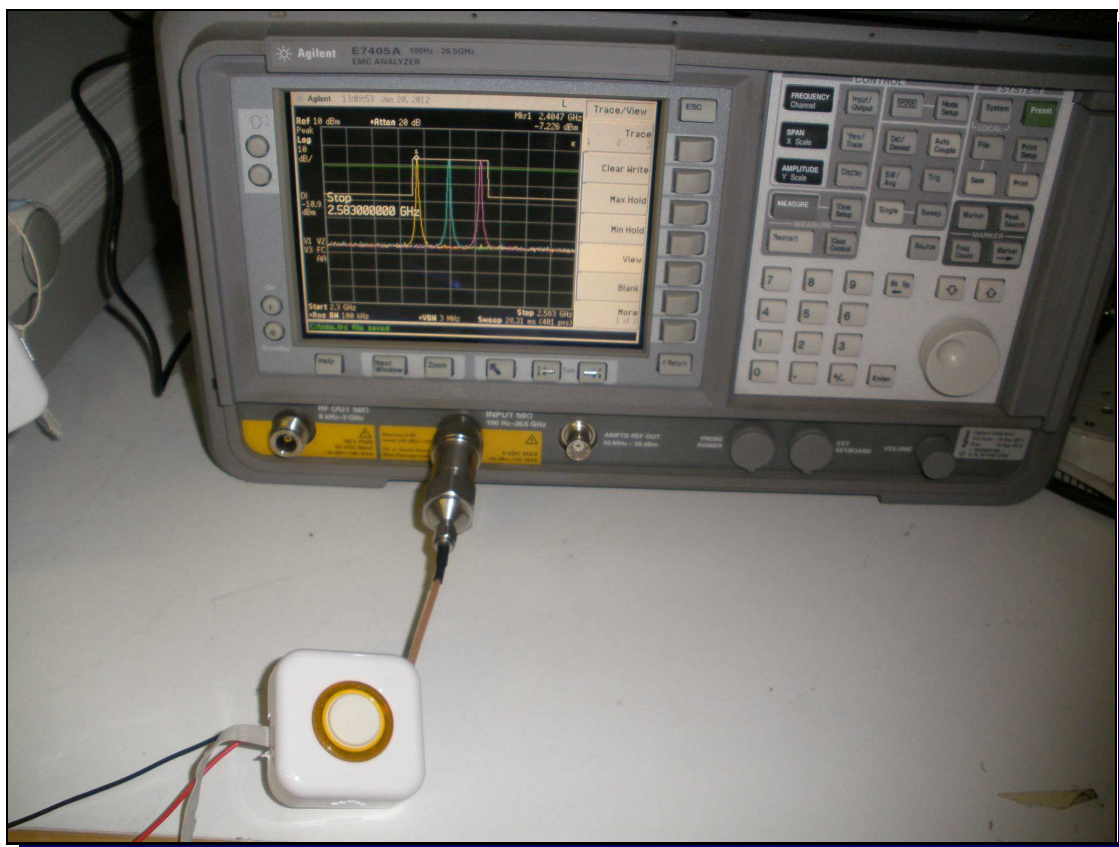
Photograph 4 Conducted Antenna
