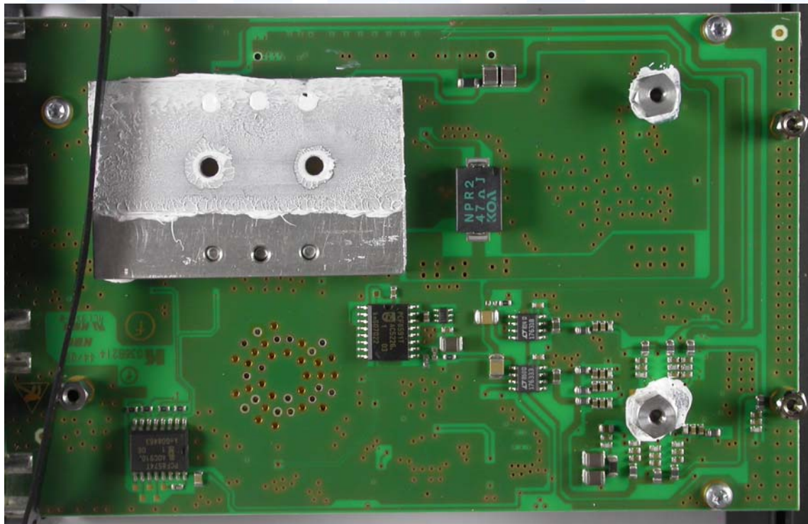
Rear view, antenna connector board
