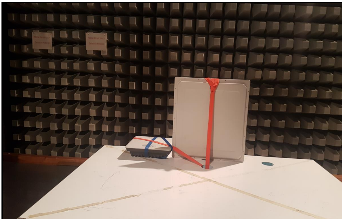
Photo 5: WIRA-40-linear-FCC Antenna
