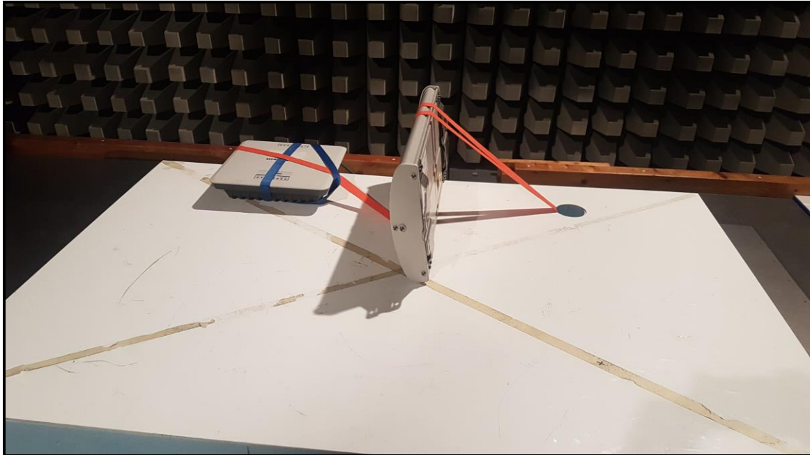
Photo 8: WIRA-30-circular-FCC Antenna
