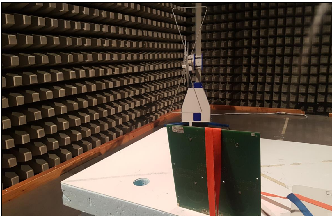
Photo 4: SSMH-30-30-ETSI-FCC Antenna
