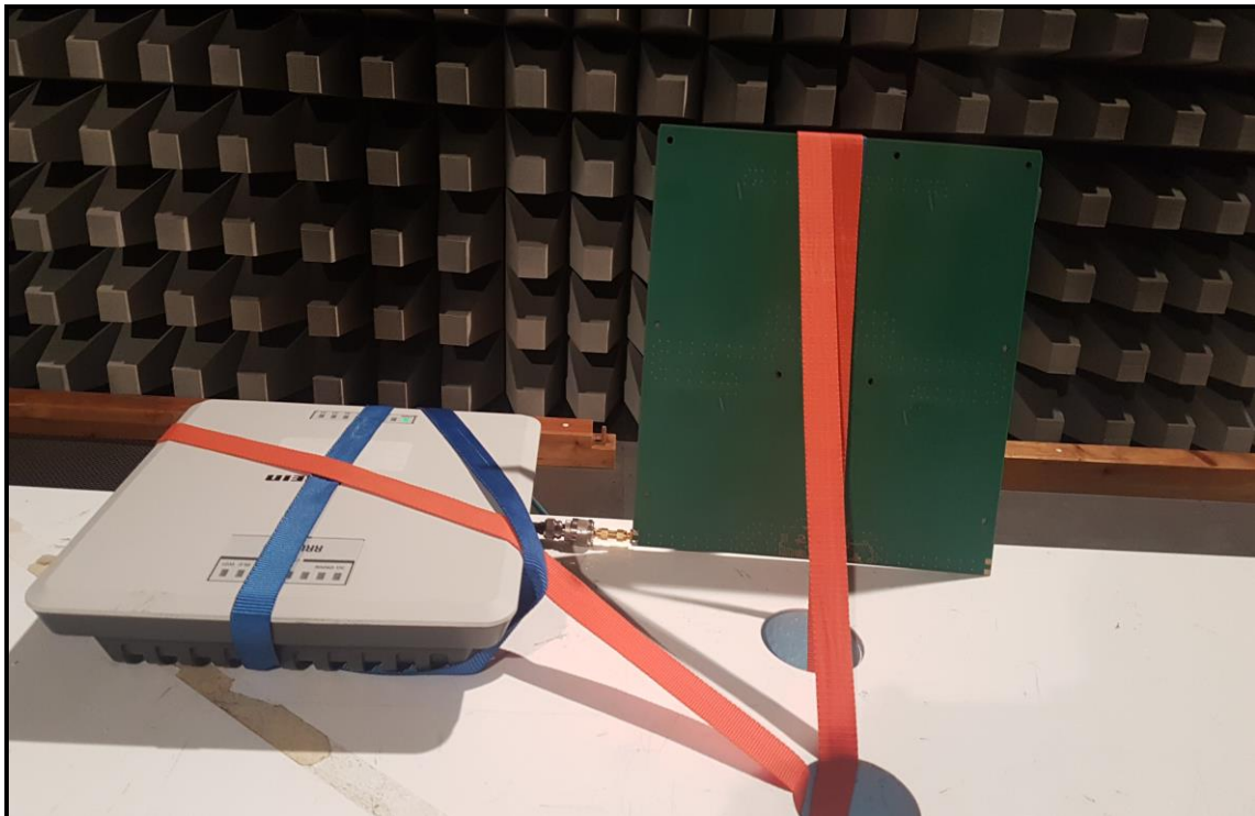
Photo 3: SSMH-30-30-ETSI-FCC Antenna
