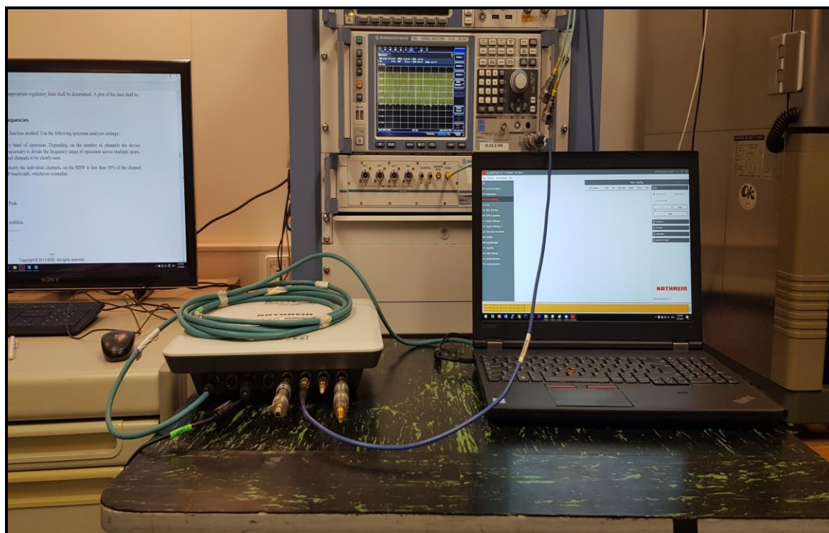
Photo 9: Conducted Tests on Port 2
