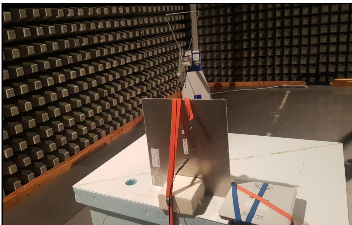
Photo 6: WIRA-40-linear-FCC Antenna
