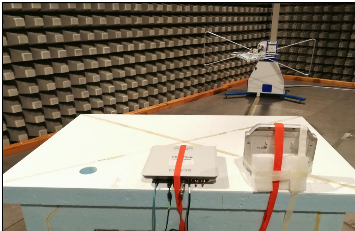
Photo 2: WIRA-70-KRAI-FCC Antenna
