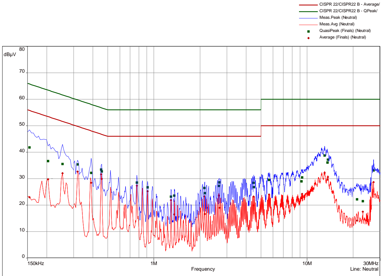
CISPR 22/CISPR22B
