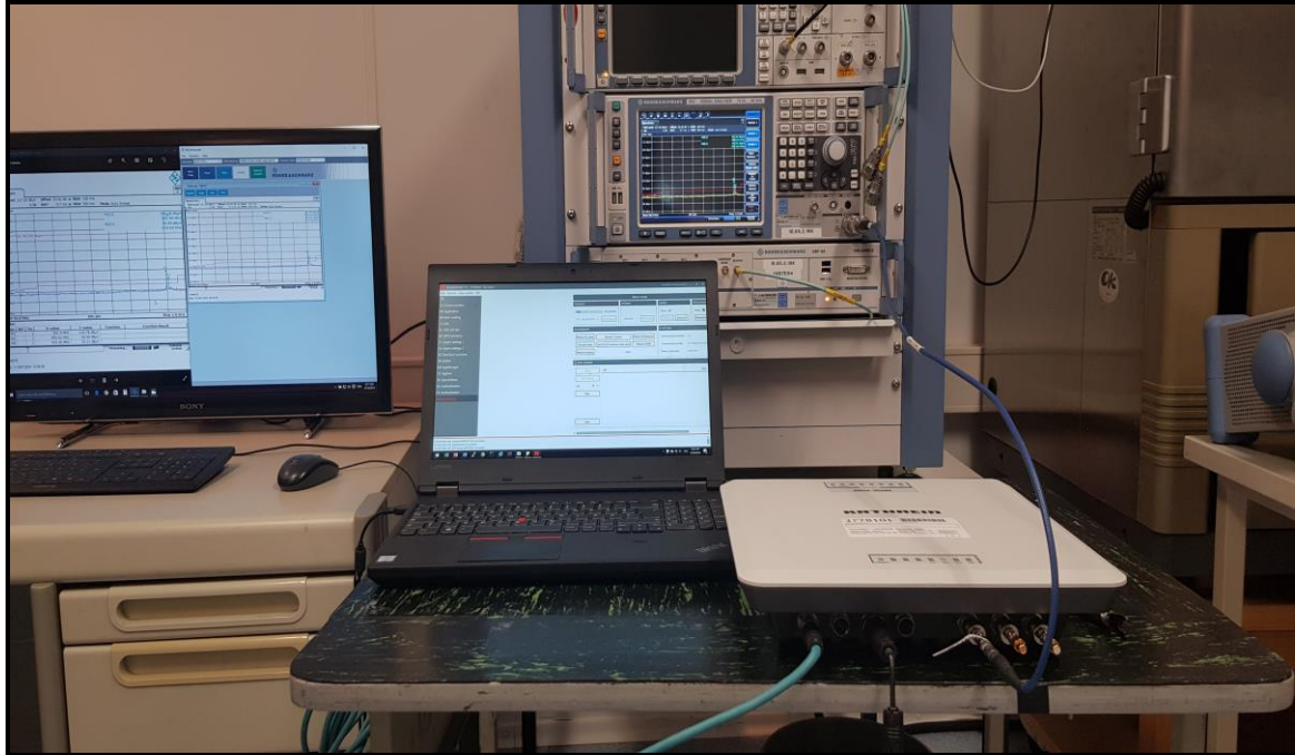
Photo 11: Conducted Tests on ARU 3500 Port 2
