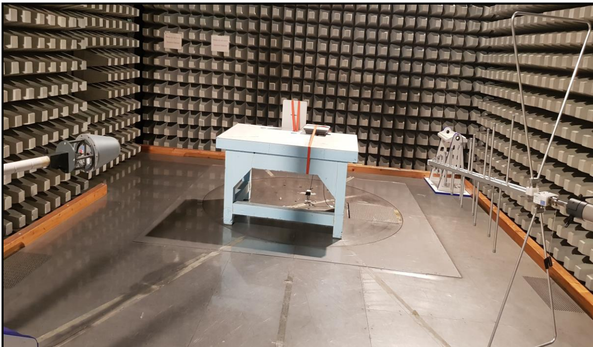
Photo 4: ARU 3560 + WRA 7070 Antenna Unit
