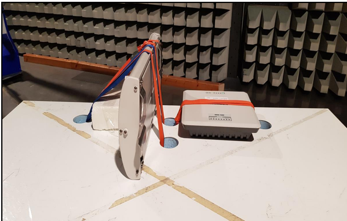
Photo 10: ARU 3560 + WIRA-30-circular-FCC Antenna
