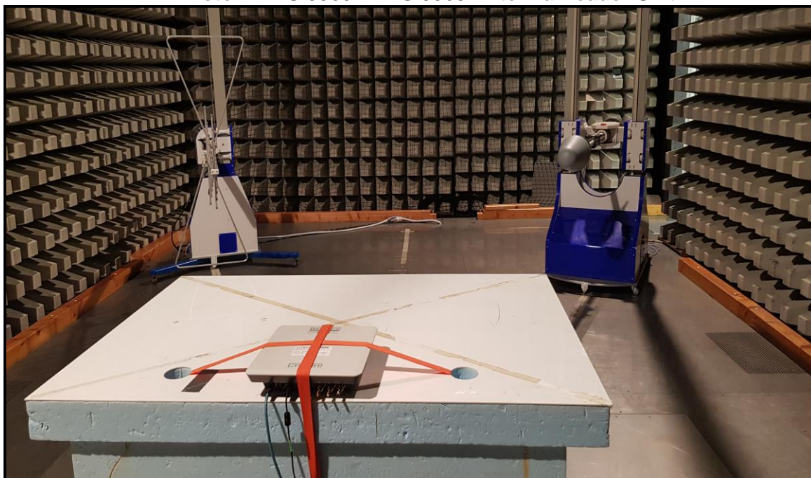
Photo 2 ARU 3560 +ARU 3560 Antenna Reader Unit
