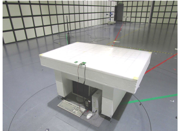
Rear (vertical)
