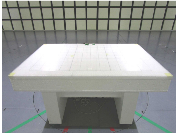
Rear (horizontal)
