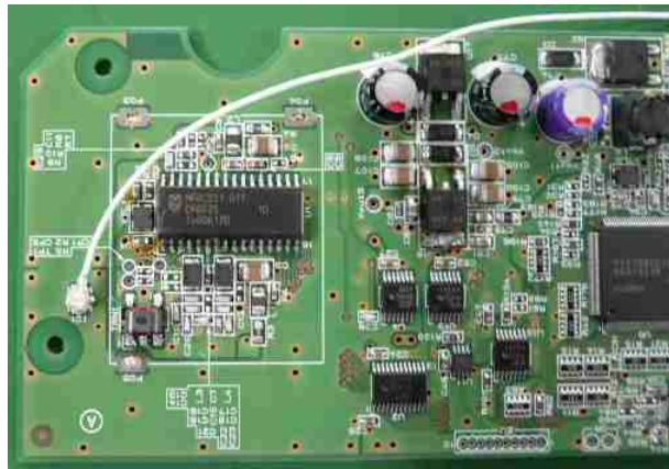
RF part substrate (without shield boards).
