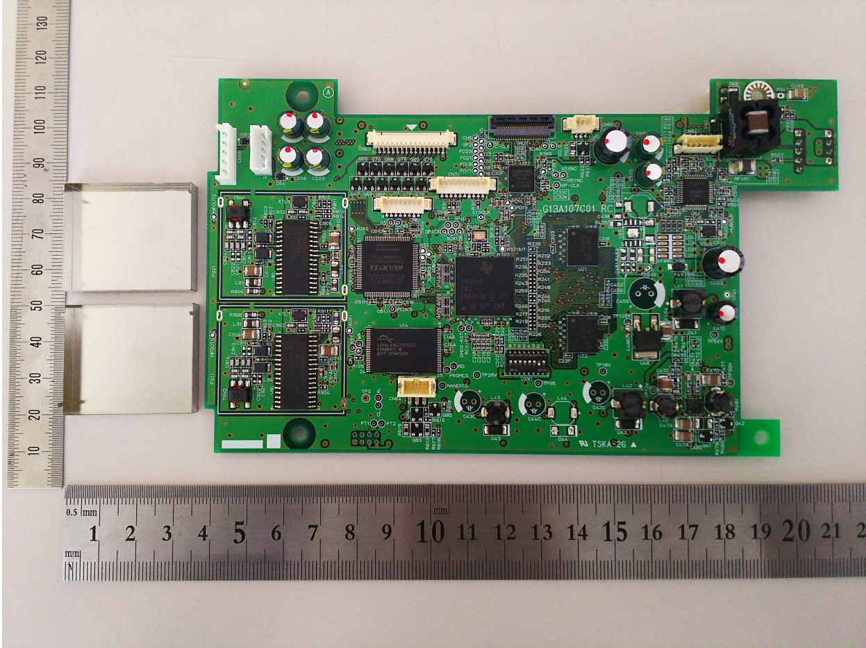
Main control board (Front side; Metal case open)
