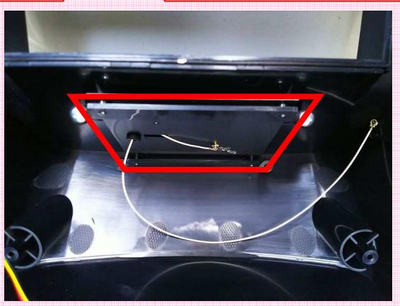
Loop antenna board (Lower antenna)
