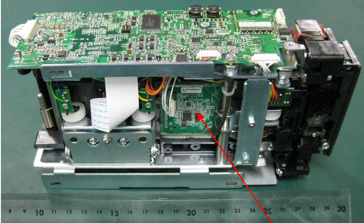
RF Circuit & Antenna Circuit Board
