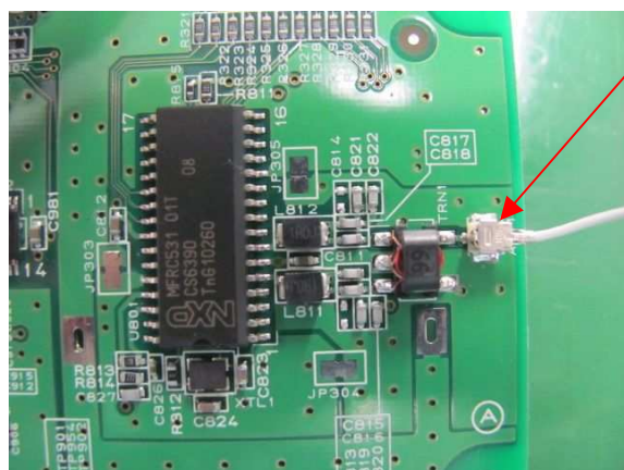
Control PWB
