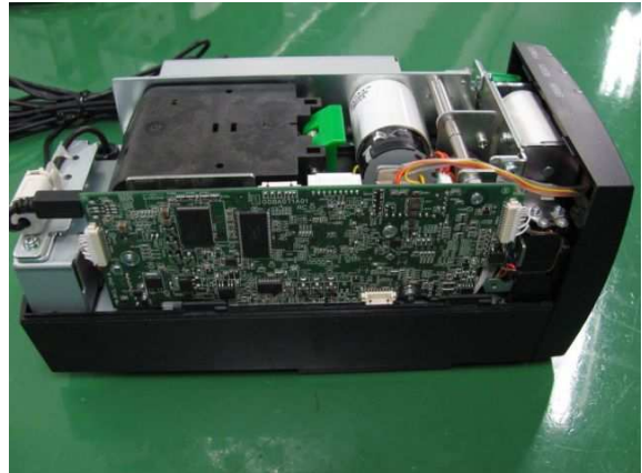
The backside of the card transportation part.
