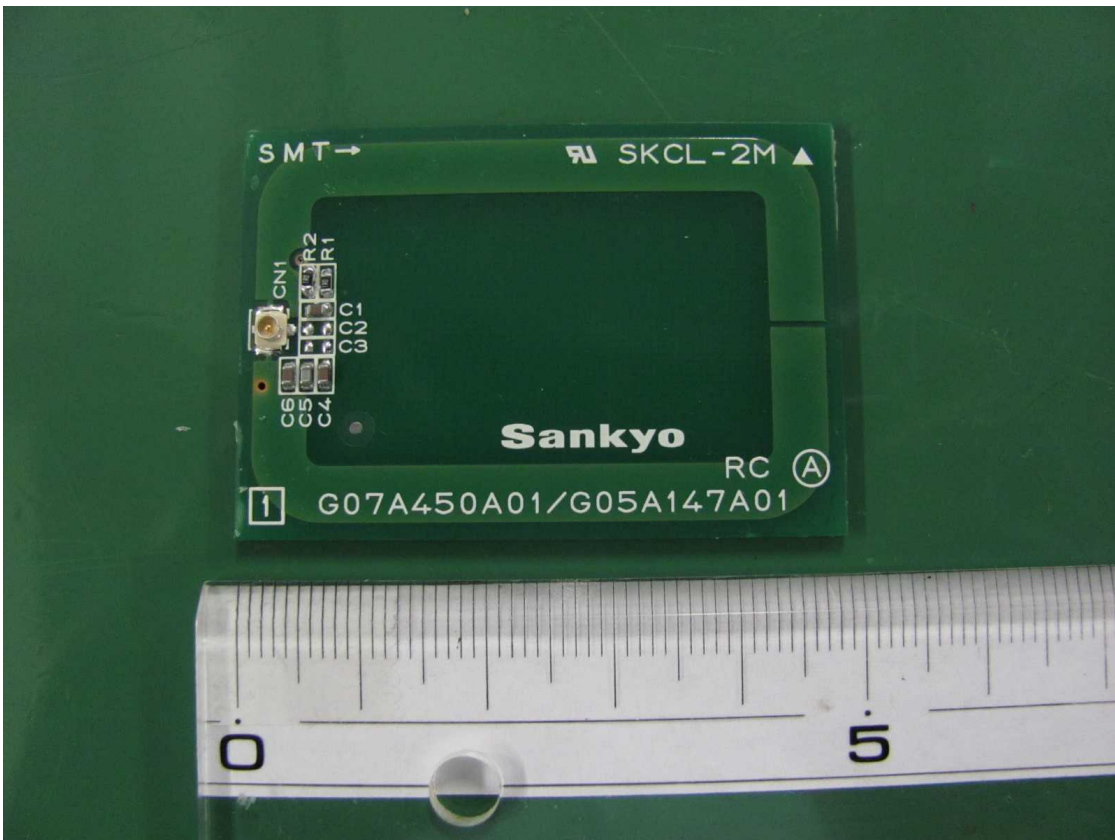
Antenna PCB (Back side)
