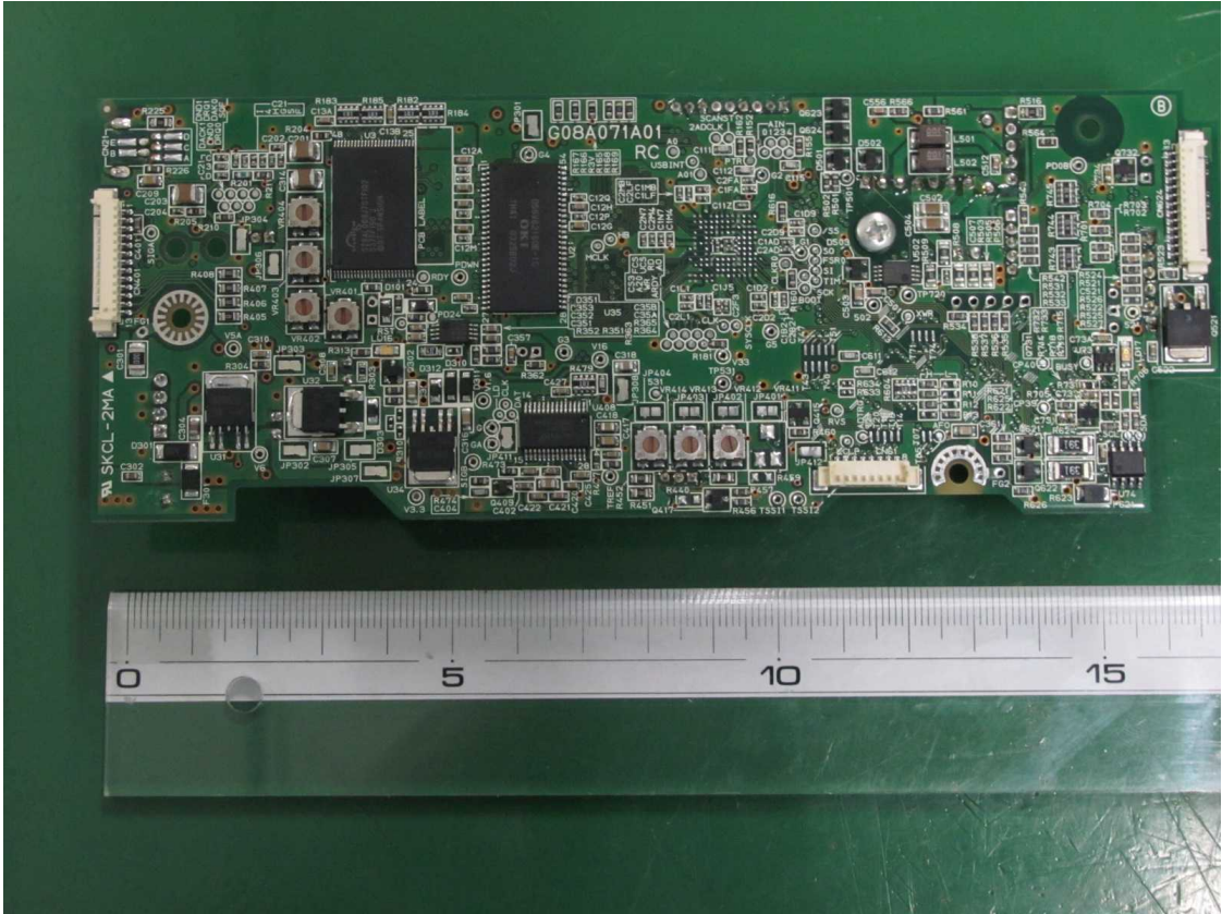
Main PCB (Surface)
