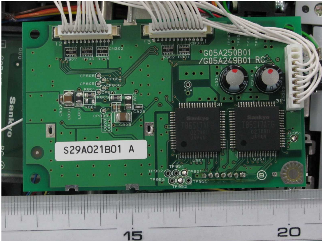
RF control PCB (Back side)
