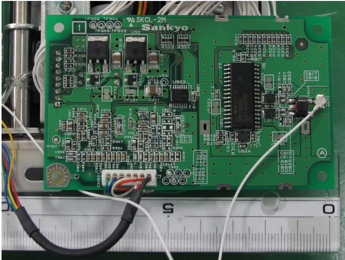
RF control PCB (Surface)
