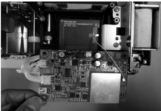
Wireless part circuit and antenna circuit
