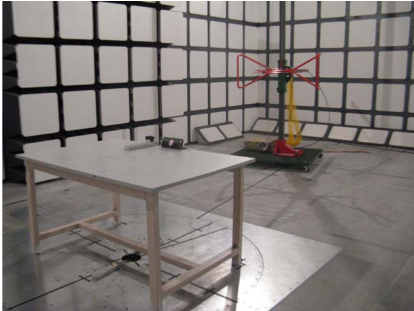
Radiated Emissions - Front View (adapter power below 1GHz)
