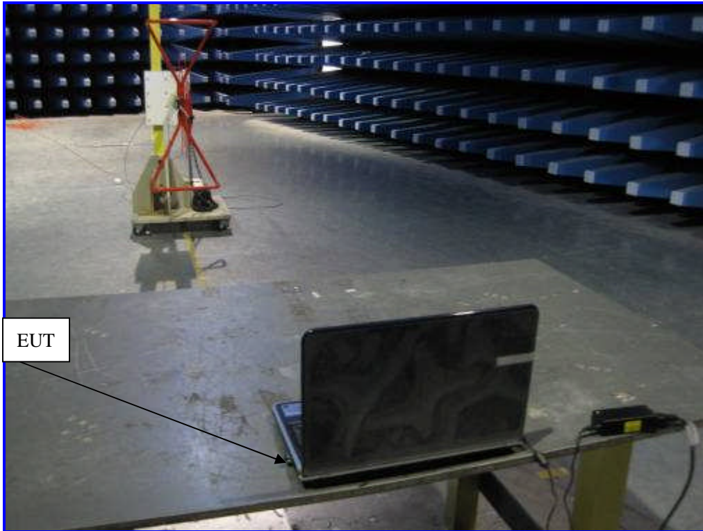
Radiated Emission Setup Rear View below 1GHz
