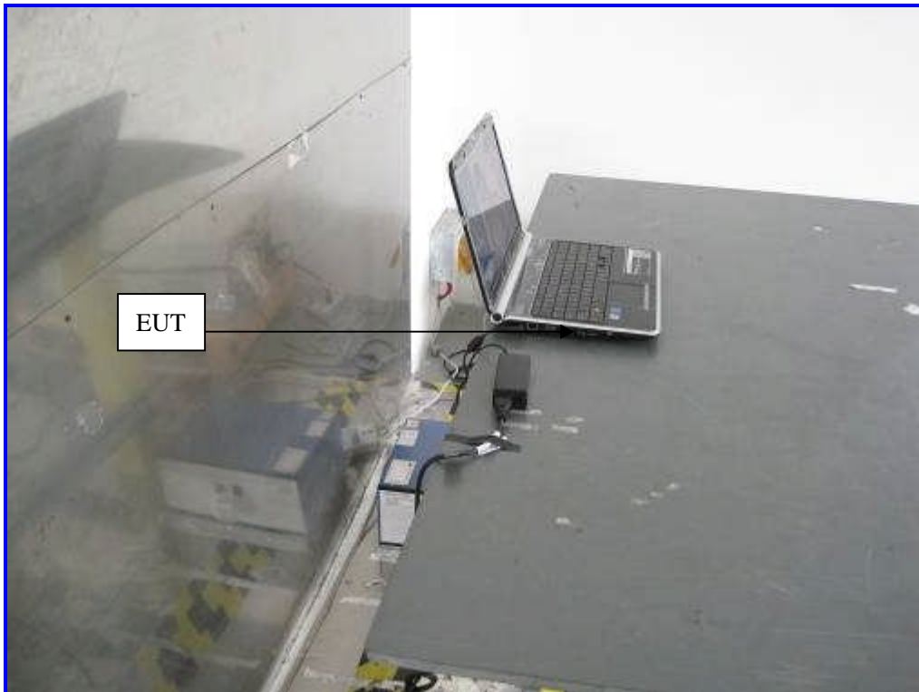
Conducted Emission Setup Side View
