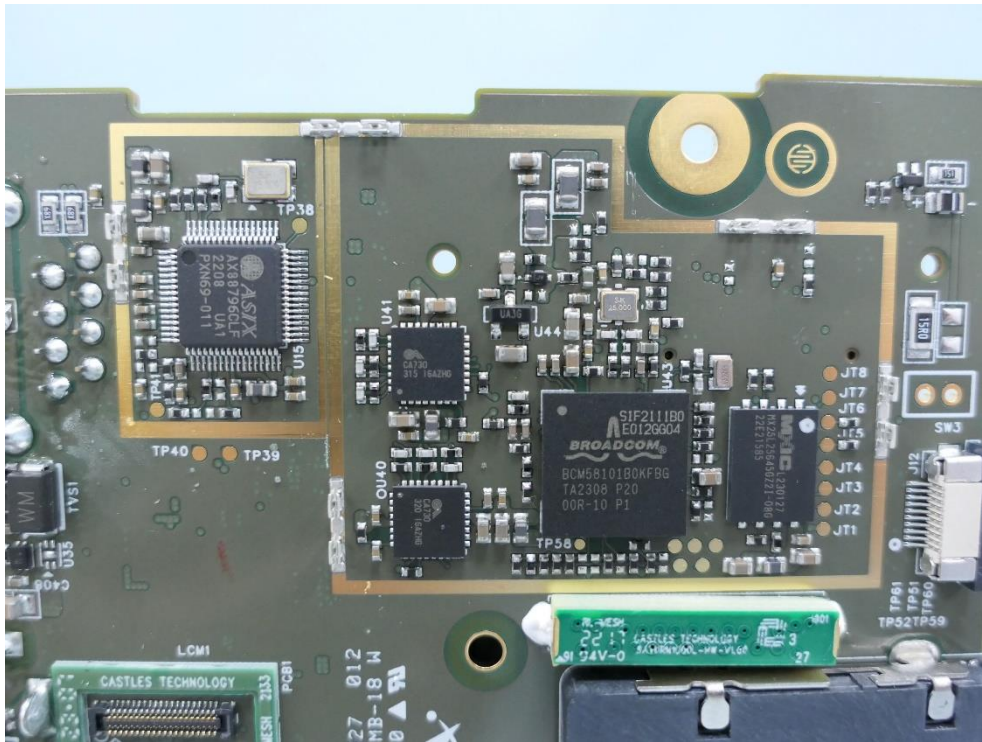
(39) EUT Photo
