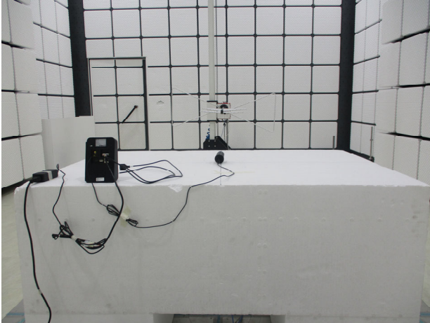
FCC_22_H_2G_Radiated_Setup
