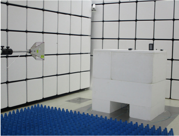
FCC_22_H_2G_Radiated_Setup
