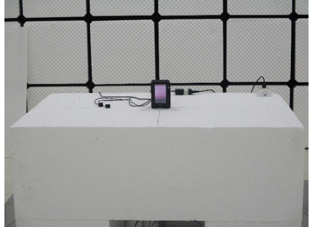
FCC_15_407_WLAN_Radiated_Setup
