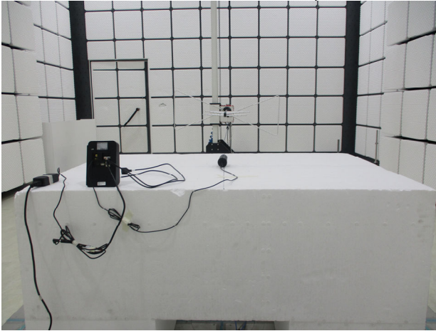
FCC_22_H_3G_Radiated_Setup
