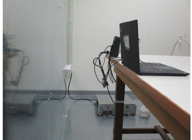
FCC_15_225_NFC_Conduction_Setup
