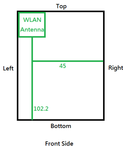
Antenna location (front side)
