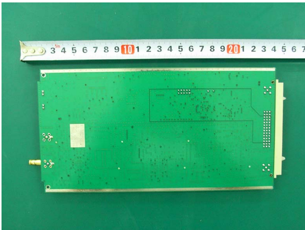
Photo of TRF Board bottom view
