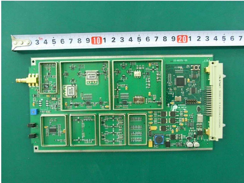
Photo of SYN Board top view
