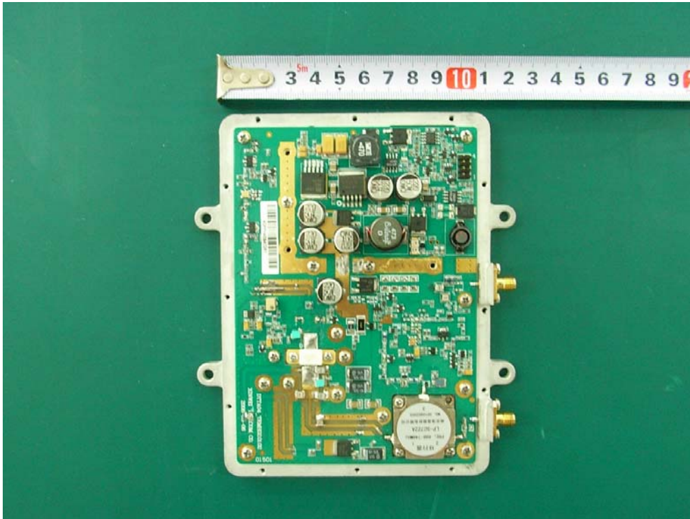
Photo of TTA PCB top view
