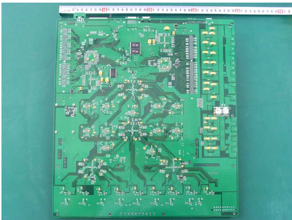
Photo of BBP Board bottom view
