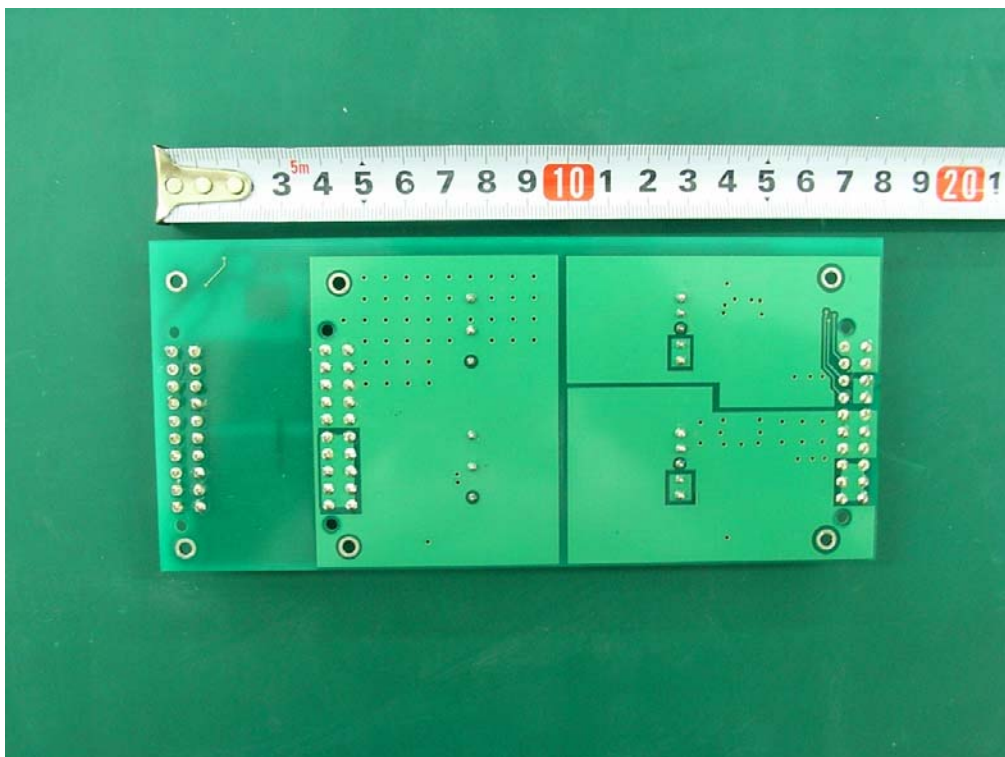
Photo of PL Board bottom view
