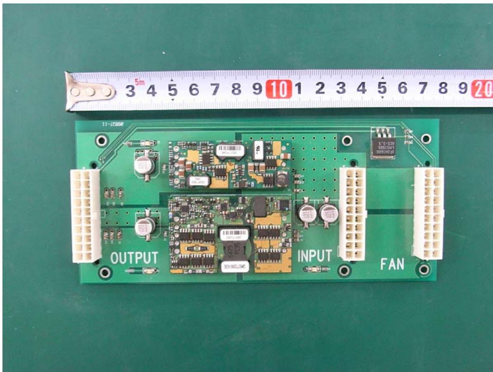
Photo of PL Board top view
