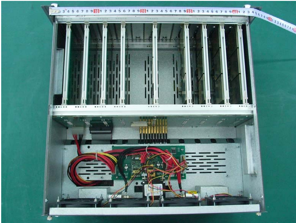
Photo of BTS inner layout
