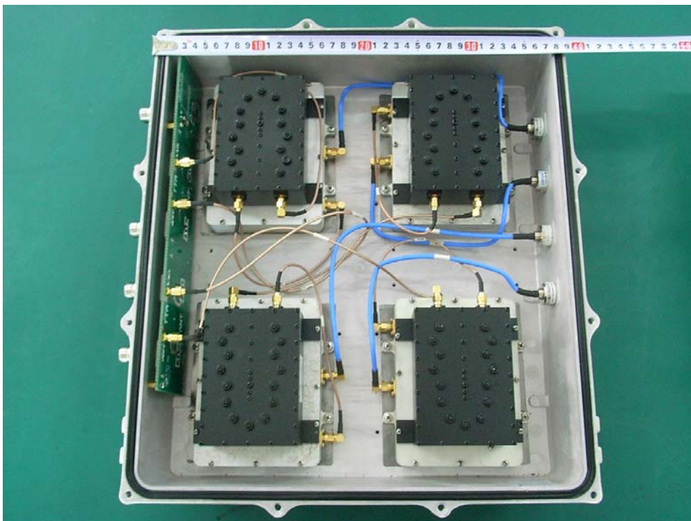
Photo of TTA inner layout
