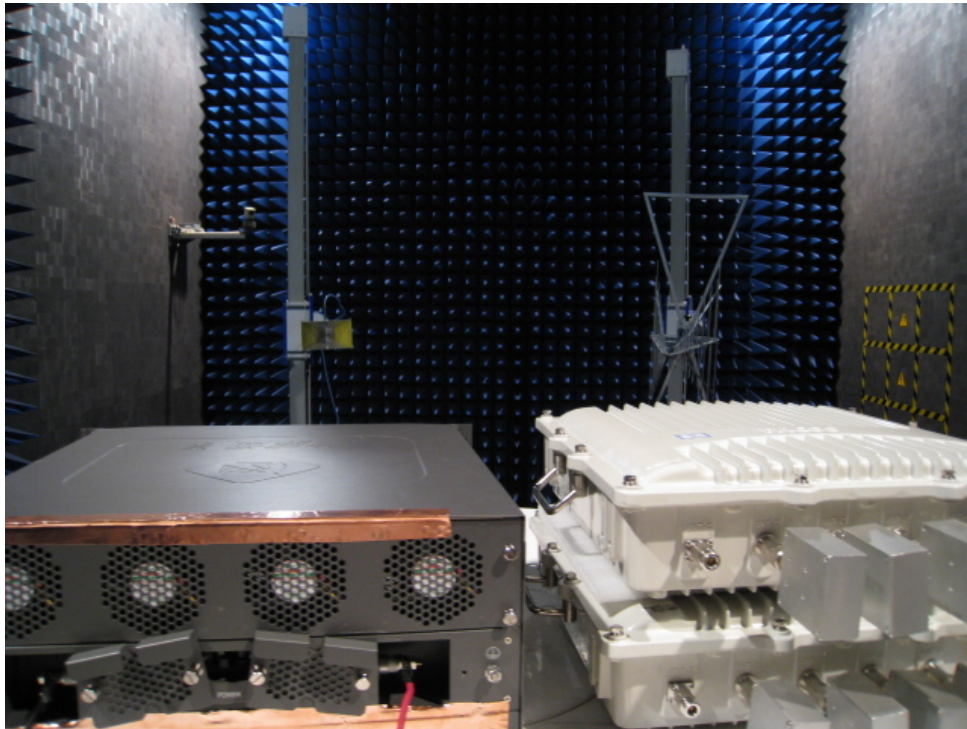
Photograph of Radiated Spurious Emissions Test Setup
