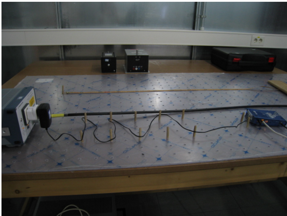
Photograph of Power line Conducted Emissions Test Setup
