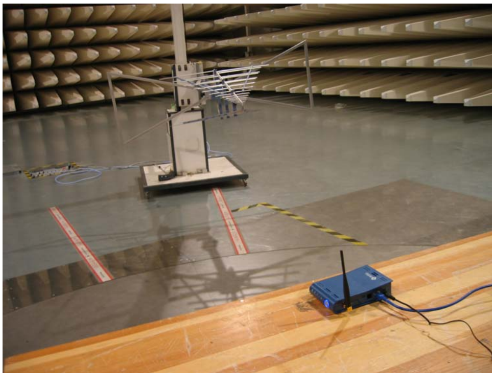
Photograph of Enclosure Radiated Emissions Test Setup
