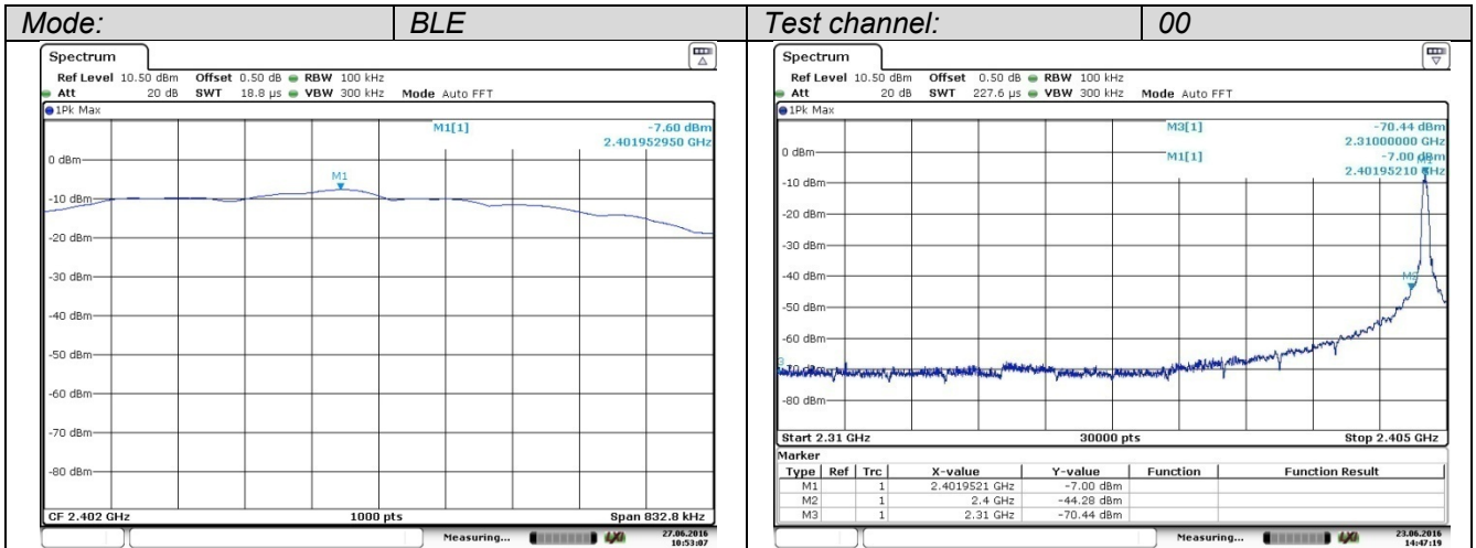
100KHz PSD Reference Level
