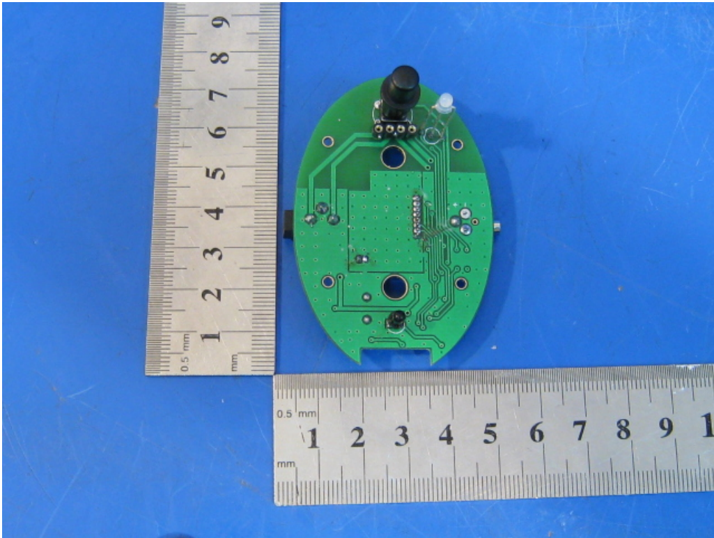
Photo 10 Inside of EUT (Transmit part)
