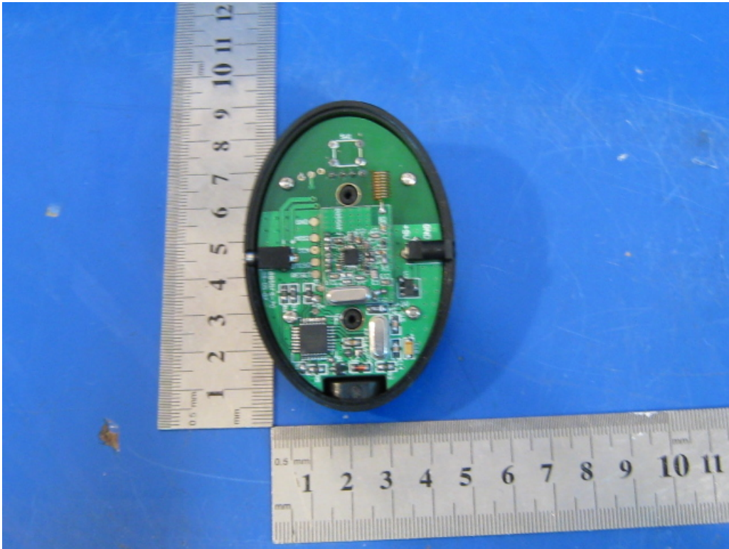
Photo 8 Inside of EUT (Transmit part)
