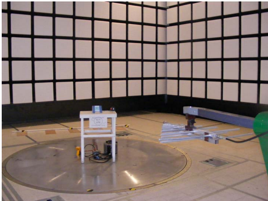
Radiated Emission with Rx/Tx mode setup photo in 3m
