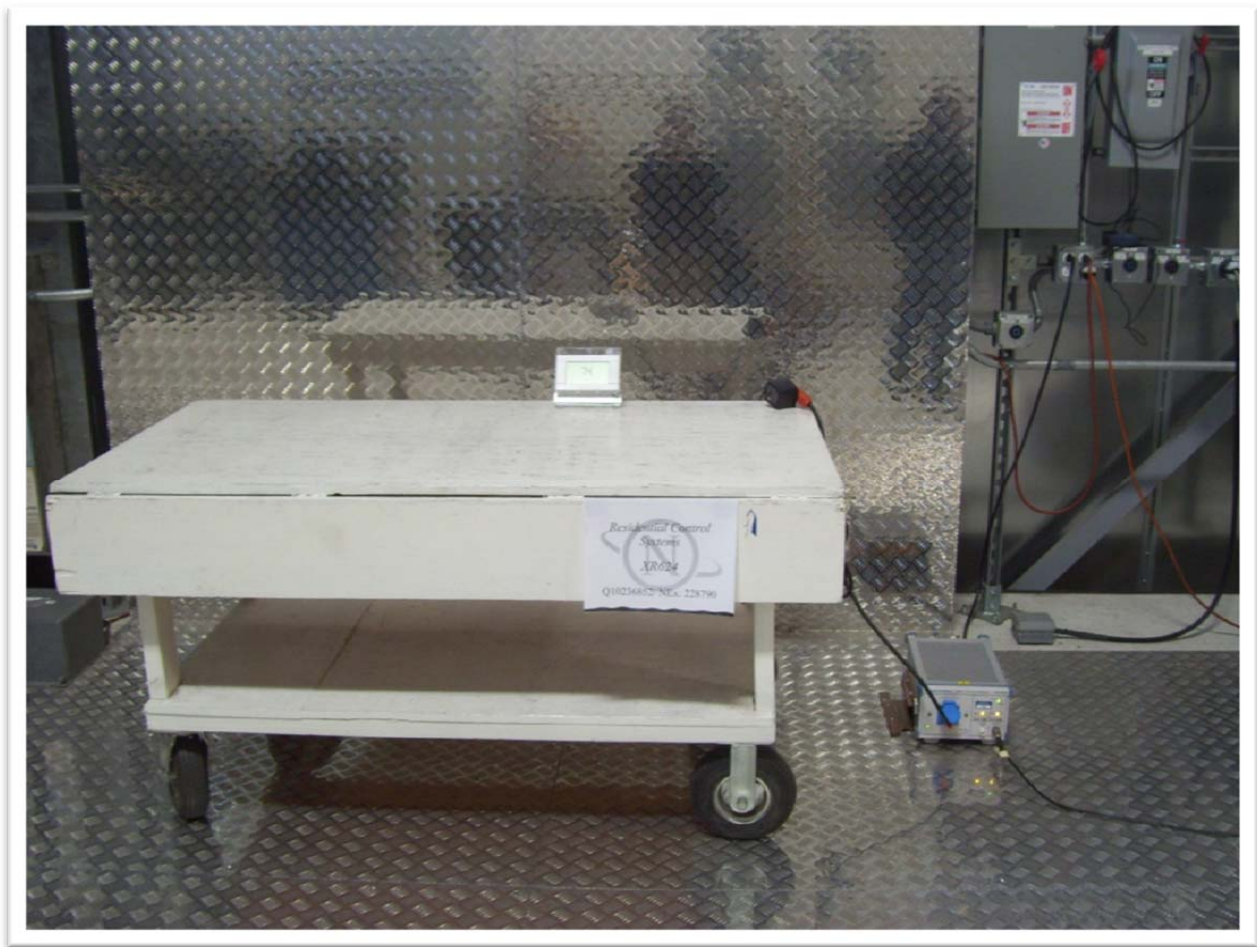
Conducted Emission setup photo
