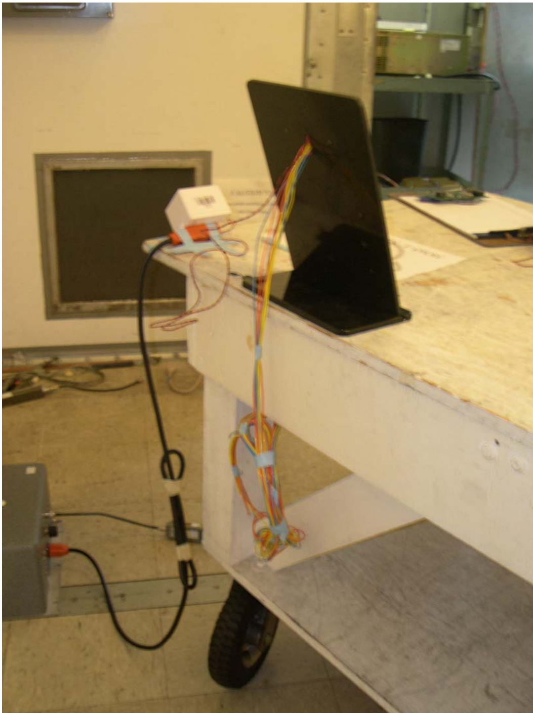
CONDUCTED EMISSIONS BACKVIEW
